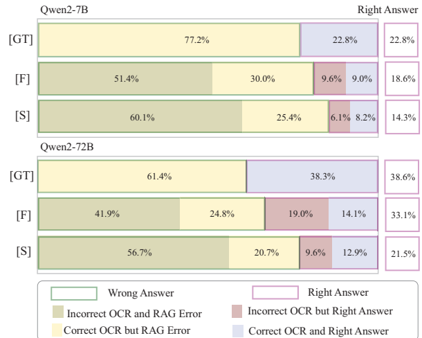
Figure 5. Analysis of answer correctness distribution in Q&A pairs, using different perturbed data and LLMs. It reveals that larger LLMs are more robust to OCR noise. [S] and [F] denote perturbed data with severe Semantic Noise and Formatting Noise , respectively. [GT] represents ground truth perturbed data.
