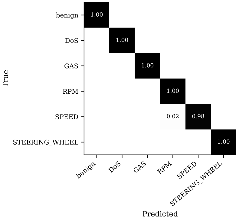
GraMa, centralised, seed 0
