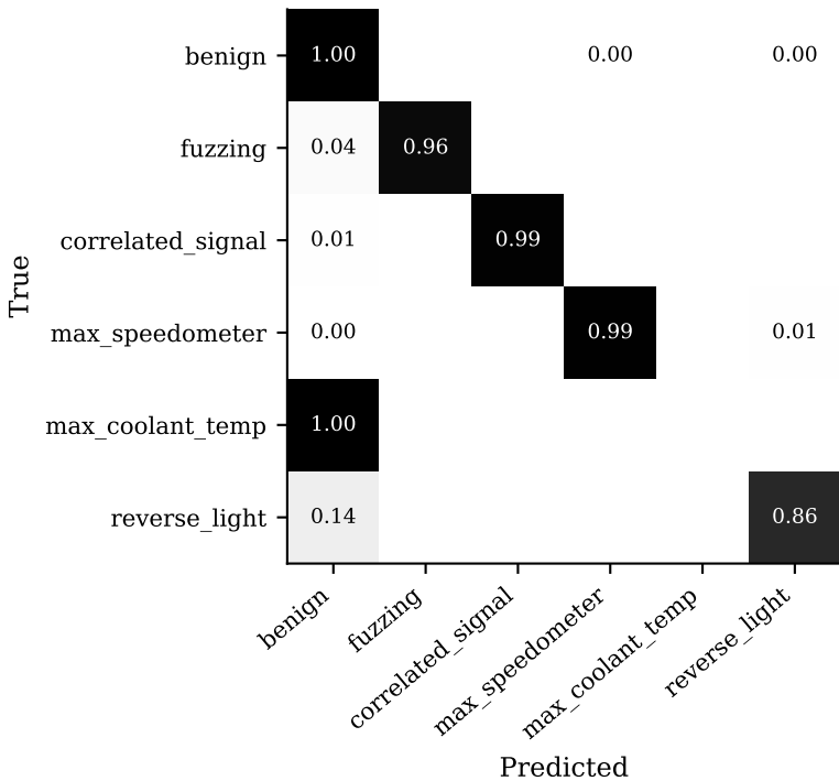
GraMa + FedAvg, seed 0
