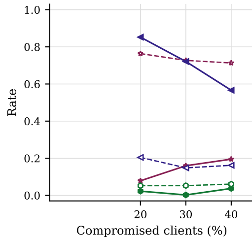
Label flipping
