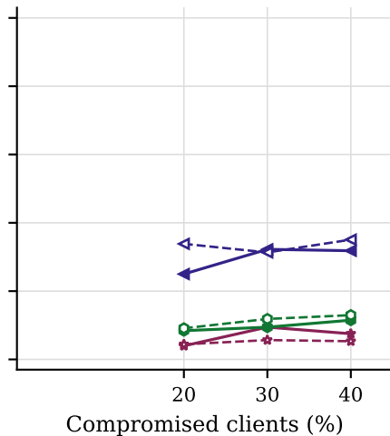
Magnitude poisoning
