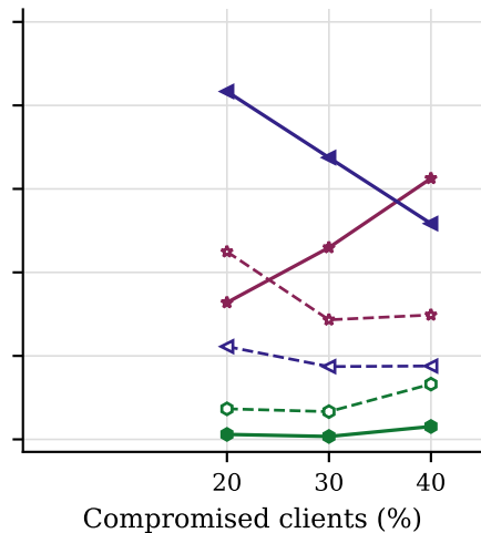
Targeted flipping
