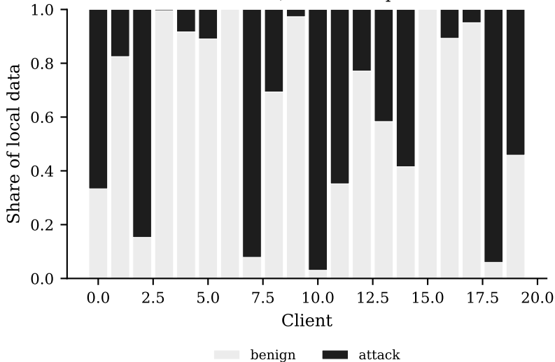
Client label mix, Dirichlet alpha = 0.5
