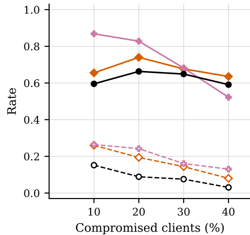
Label flipping
