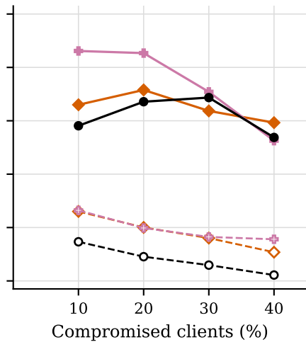
Targeted flipping
