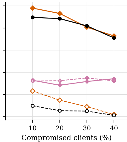
Magnitude poisoning
