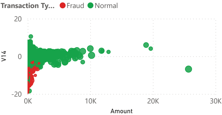
risk analysis
