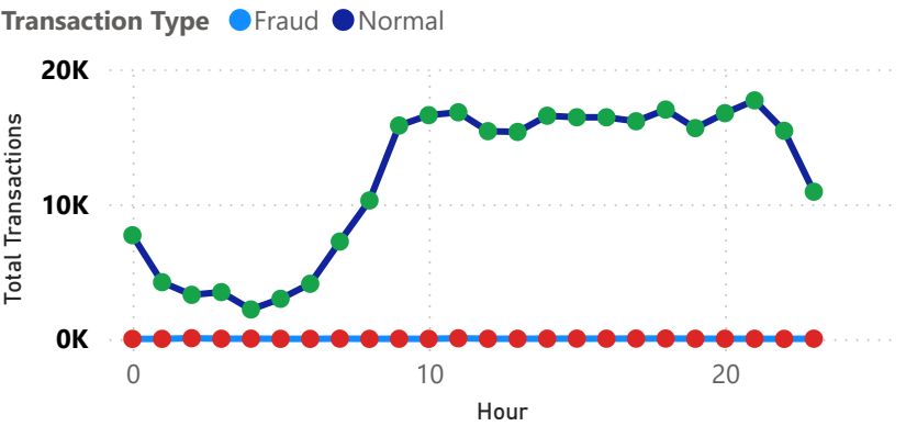
fraud trend
