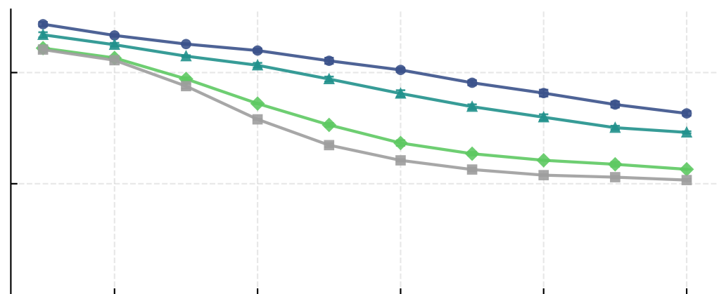
Non-equatorial hot-spot orbits
