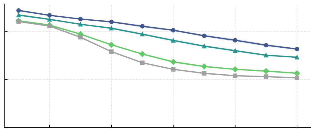
Non-equatorial hot-spot orbits
