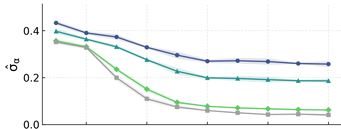
Equatorial hot-spot orbits
