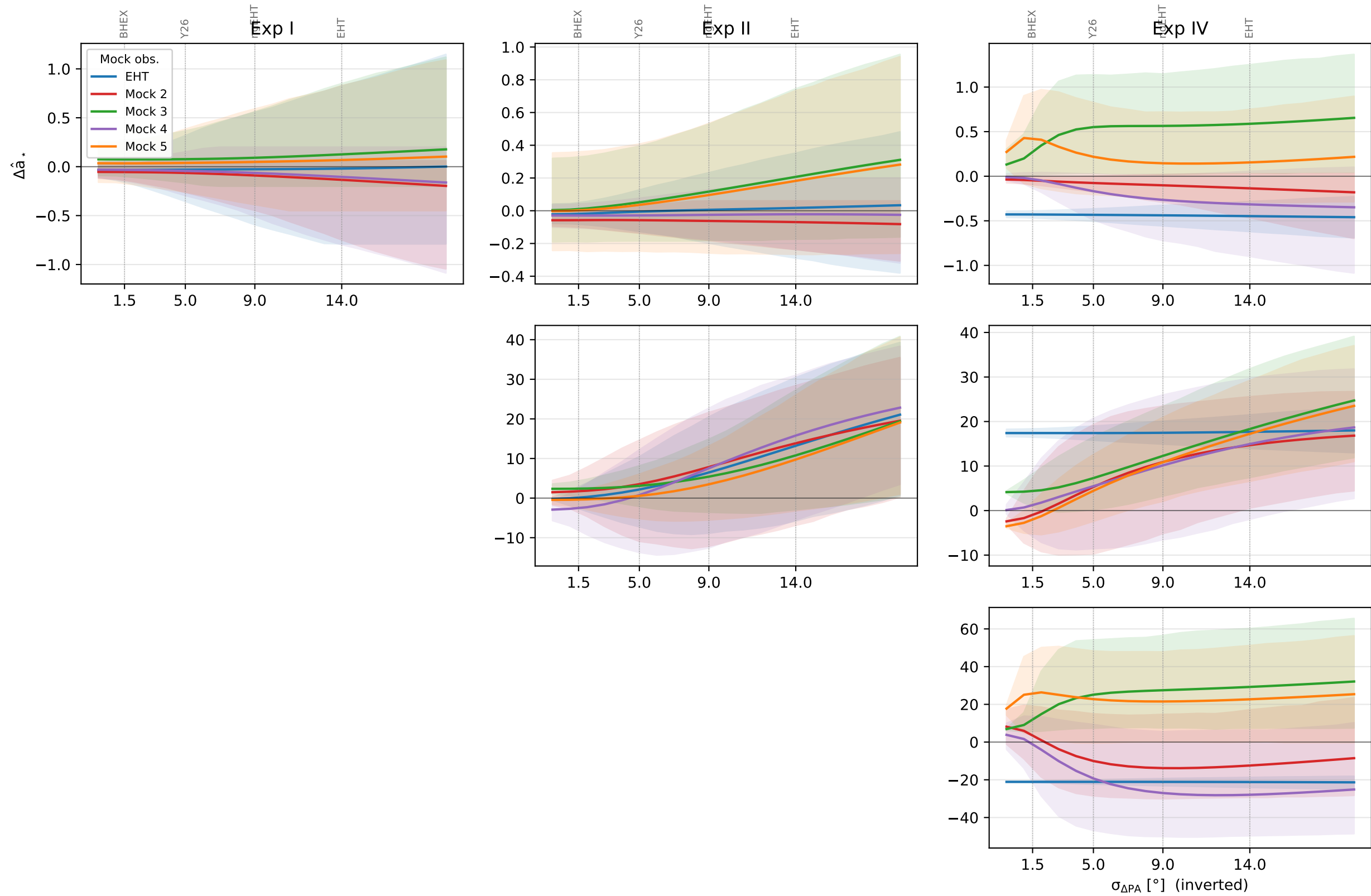
Per-mock error (prediction – truth) \pm 2\sigma band, by experiment (cols) and target (rows)
