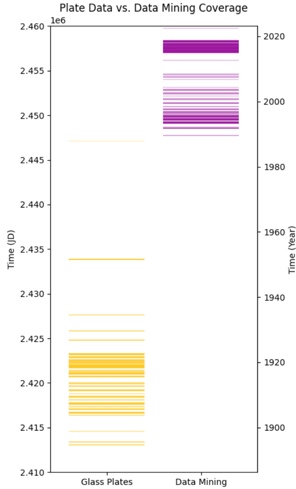
Figure 8: KZ Her Event Plot of Yerkes Plates vs. AAVSO, Gaia, and ASAS-SN Data
