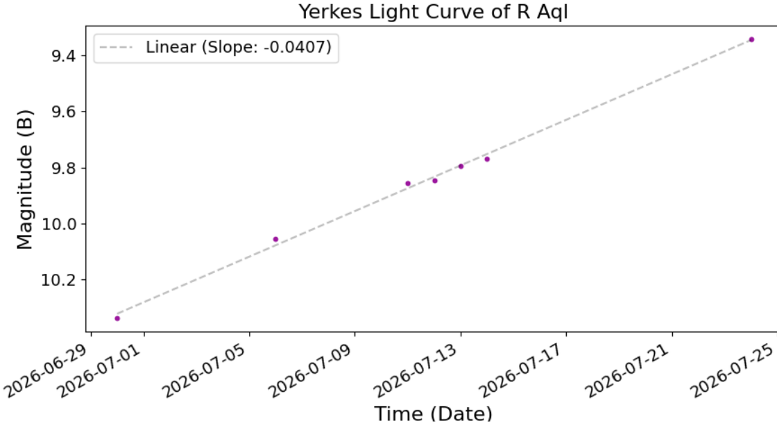
Figure 7: Light Curve of R Aql from 24-in Reflector with curve fit
