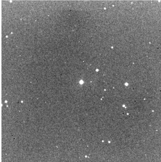
Figure 6: R Aql centered in 60s exposure in B band
