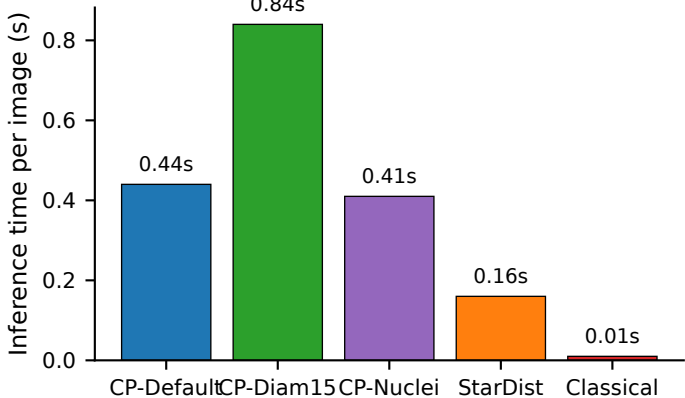
Computational cost (V100 GPU; CL on CPU)
