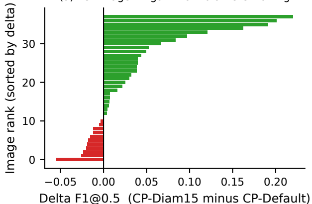
(a) Per-image F1 gain from diameter tuning
