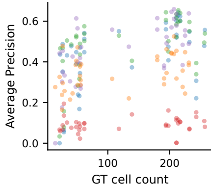
(c) Average Precision ( r=0.33 , p=0.000 )
