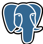
FIGURE 4.3 – Logo PostgreSQL
