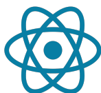
FIGURE 4.4 – Logo React
