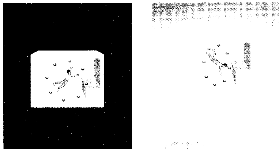
FIGURE 21.2 The two observers of Figure 21.1 after a little time. The unaccelerated particles in empty space have remained in a circle. The different accelerations of the test particles falling toward the planet have distorted the initial circle into an ellipse. In this way the freely falling observer can detect tidal gravitational accelerations if the laboratory is big enough to allow measurable differential accelerations between the test particles.
