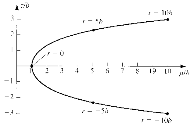
FIGURE 7.4 The curve \rho = b \cosh(z/b) , which when rotated around the z -axis, generates the two dimensional surface shown in Figure 7.5, which has the same intrinsic geometry as (7.41), and is thus an embedding of an (r, \phi) slice of the wormhole geometry (7.39) in three-dimensional flat space.
