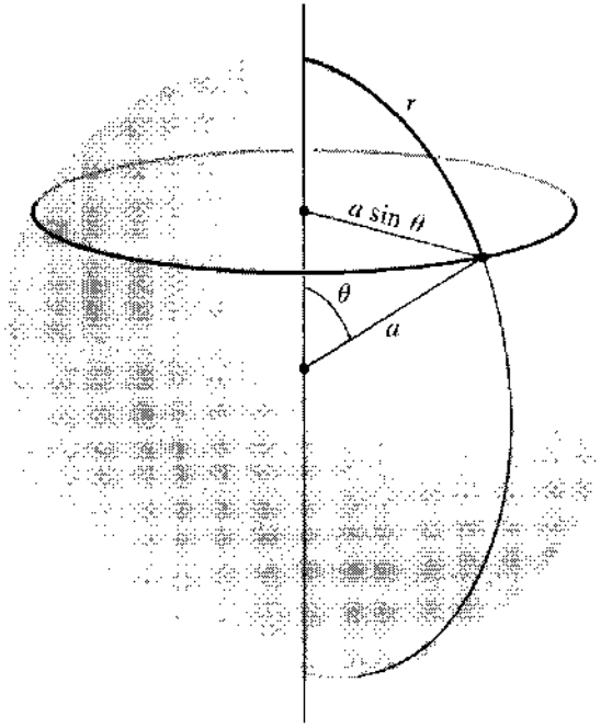
FIGURE 2.4 The relation of the circumference to the radius of a circle in the geometry of the surface of a sphere. A circle is the locus of points on the surface that are equidistant (as measured on the surface) from its center point. In this figure the North Pole has been chosen to coincide with the center of a circle that is a line of constant latitude labeled by \theta . The radius r is the distance from the North Pole to this latitude measured along any line of constant longitude.
