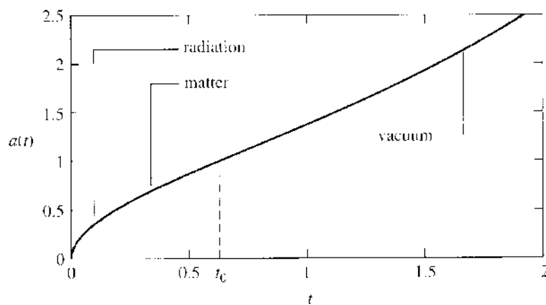
FIGURE 18.4 Stages of evolution in a flat FRW model. The various stages in the expansion of a flat FRW model are shown in this figure for the \Omega_r = \Omega_m = \Omega_v = \frac{1}{3} illustrative model whose effective potential is shown in Figure 18.3. At early times the expansion is radiation dominated ( a(t) \propto t^{1/2} ), later matter dominated ( a(t) \propto t^{2/3} ), and finally vacuum dominated ( a(t) \propto \exp(Ht) ). The present age, t_0 , when a(t_0) = 1 with our choice of normalization, is at the time of the dotted vertical line. This curve was calculated with the Mathematica program for general FRW models available on the book website.
