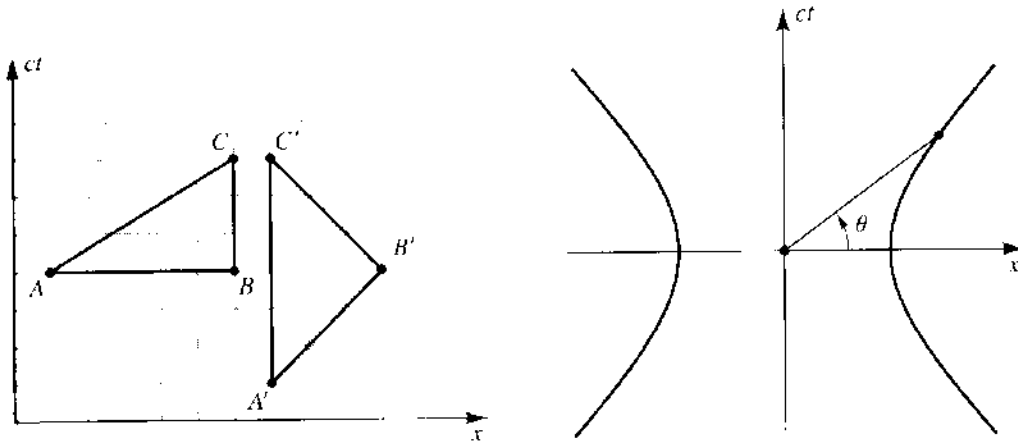
FIGURE 4.8 A little spacetime geometry. The left-hand figure shows a spacetime diagram with two triangles whose properties are discussed in the text. The right-hand figure shows a spacetime analog of a circle—a hyperbola that is a constant spacetime distance from the origin. A hyperbolic angle \theta is a ratio of a distance along these hyperbolas to the distance from the origin. The hyperbolic angle \theta shown is the ratio of the spacetime distance along the hyperbola from the x -axis to the spacetime distance of the hyperbola from the origin.
