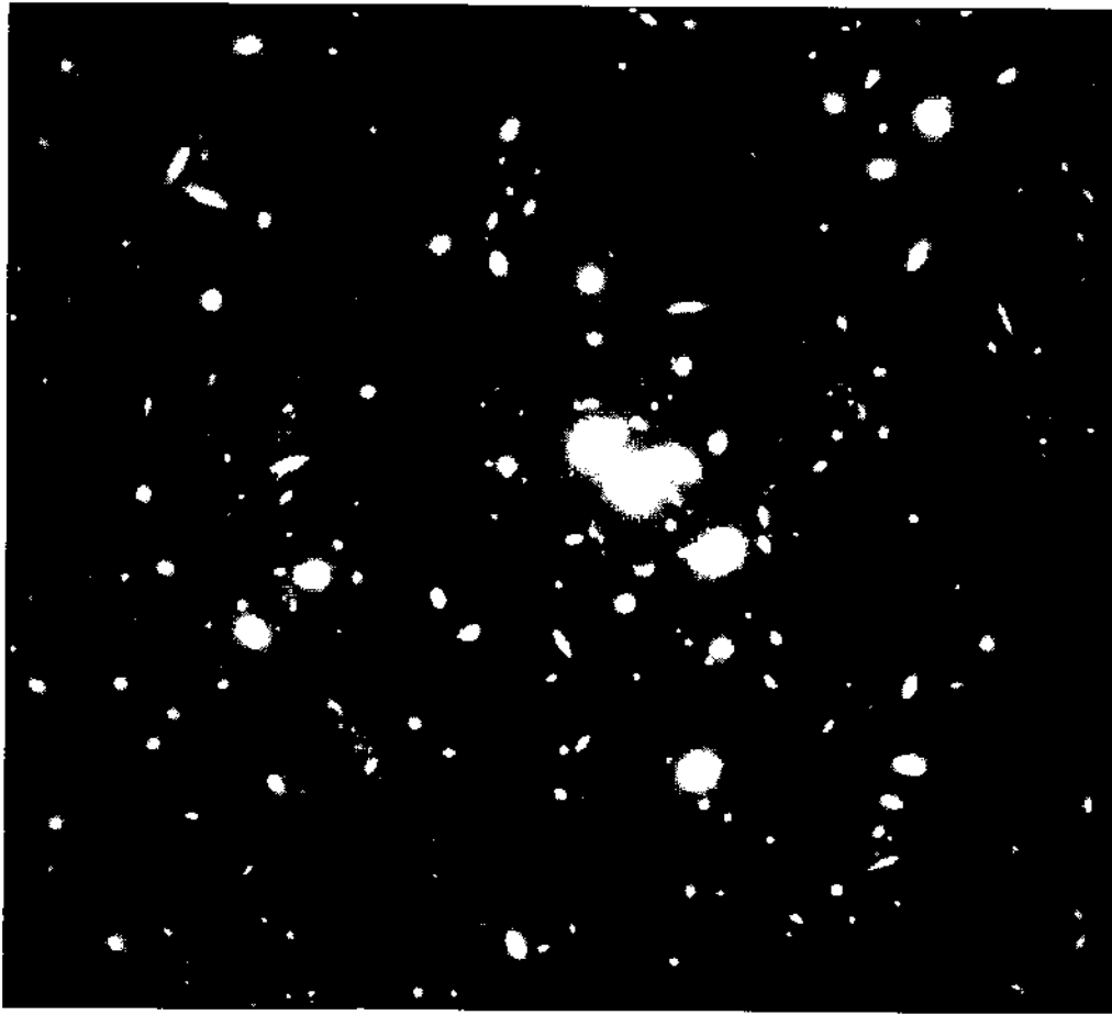
FIGURE 11.4 A Hubble space telescope image of the galaxy cluster 00244-1654 acting as a gravitational lens. The mass in the foreground cluster of galaxies (the bright, diffuse images in the center) acts as a gravitational lens for a more distant galaxy. The geometry of the lens (not a point) is such that multiple images of the distant galaxy are produced close to the radius of the Einstein ring. The images are distorted into arcs.
