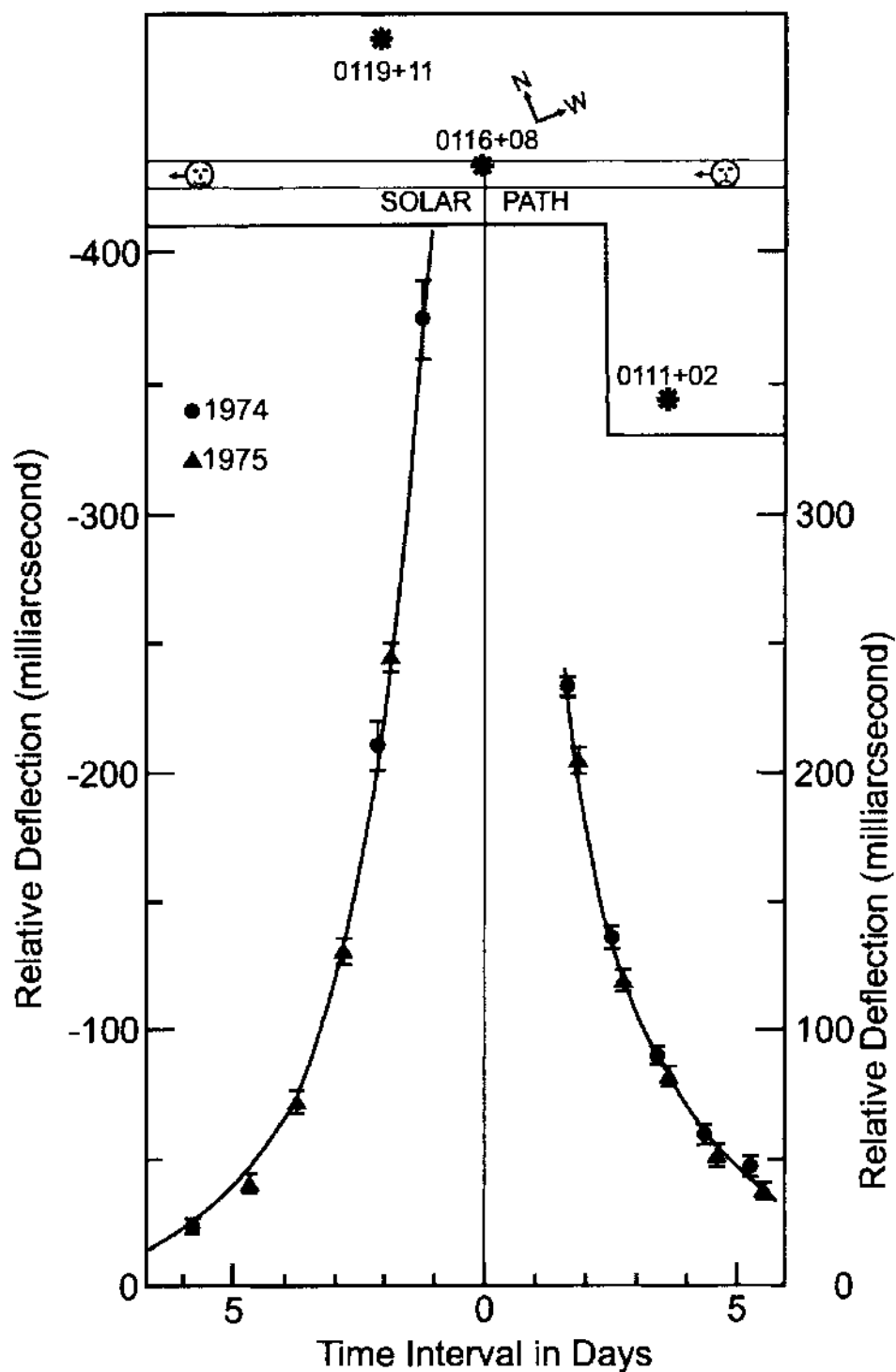
FIGURE 10.6 The deflection of the light from the radio source 0116 + 08 as a function of time as it is occulted by the Sun. The top part of this figure illustrates the path of the Sun on the sky and the relative positions of the three radio sources involved. The bottom part shows the experimental data for the deflection in angular position of 0116 + 08 measured relative to the other two sources. The solid curve is the prediction of general relativity.
