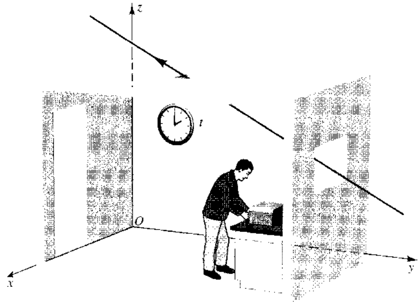
FIGURE 3.1 A laboratory defines a reference frame. An observer in an idealized laboratory can choose one corner as the origin of three Cartesian coordinates ( x, y, z ) that coincide with the intersections of the walls and floor that meet in that corner. These three coordinates define a reference frame that, together with the time measured by a clock, can be used to describe the motion of particles moving through the laboratory and state Newton's laws of motion.
