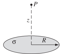
(c) Uniform surface charge
