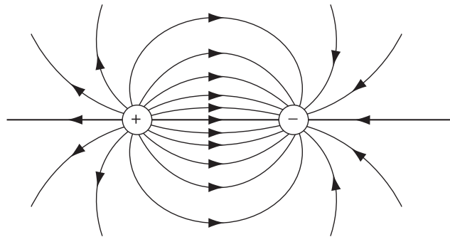
Opposite charges
