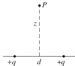
(a) Two point charges
