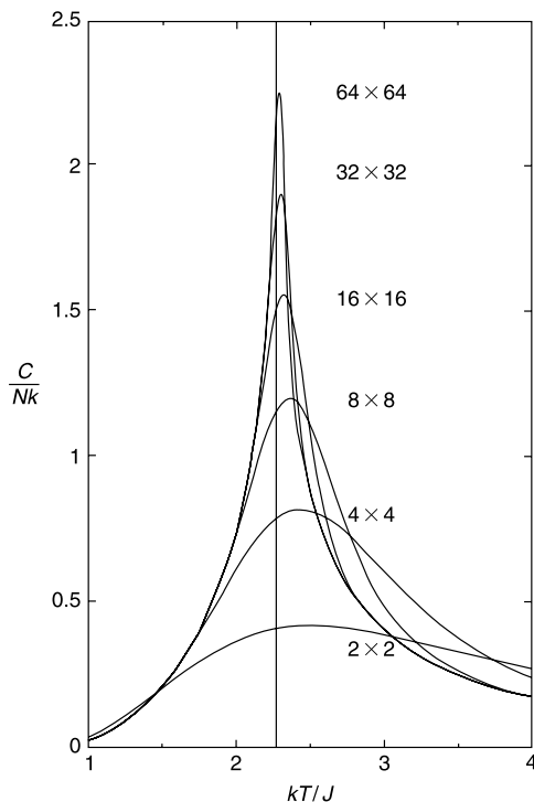
FIGURE 13.17 Specific heat of the two-dimensional Ising model for finite 2 \times 2 , 4 \times 4 , ..., 64 \times 64 lattices. The specific heat is analytic for all finite lattices. The maximum value of the specific heat grows proportional to the logarithm of the linear dimension of the lattice and the location of the maximum approaches the bulk critical temperature (denoted by the vertical line) proportional to the inverse of the linear dimension of the lattice. From Ferdinand and Fisher (1969). Reprinted with permission; copyright © 1969 American Physical Society.
