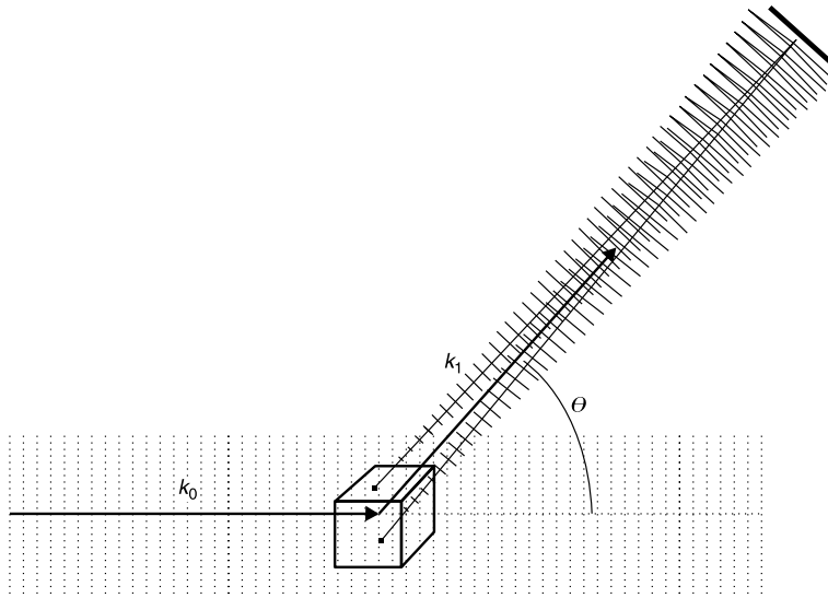
FIGURE 10.7 Scattering from two particles. The incident wave vector is \mathbf{k}_0 , the scattered wave vector toward the detector is \mathbf{k}_1 , and the wave vector transfer is \mathbf{k} = \mathbf{k}_1 - \mathbf{k}_0 . Since |\mathbf{k}_1| = |\mathbf{k}_0| for quasielastic scattering, the magnitude of the wave vector transfer is k = 2k_0 \sin(\theta/2) , where \theta is the angle between \mathbf{k}_0 and \mathbf{k}_1 .
