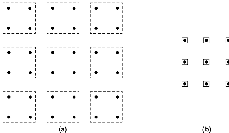
FIGURE 14.1 A block-spin transformation, with l = 2 and d = 2 . (a) The original lattice has N (= 36) spins. (b) The transformed lattice (b) has N' (= 9) spins. After rescaling, the latter looks very much the same as the former, especially in the limit N, N' \rightarrow \infty .
