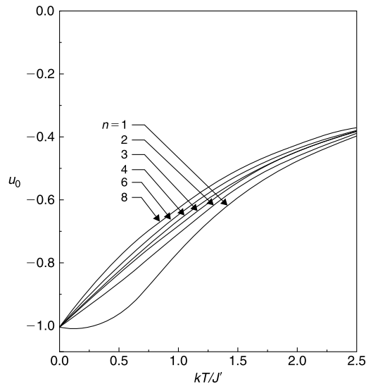
FIGURE 13.6 The normalized energy u_0 (= U_0/NnJ') of a one-dimensional chain as a function of the temperature parameter kT/J' for several values of n (after Stanley, 1969a,b). Note that for this classical model, the slopes as T \rightarrow 0 are given by the equipartition theorem for n - 1 degrees of freedom per spin.
