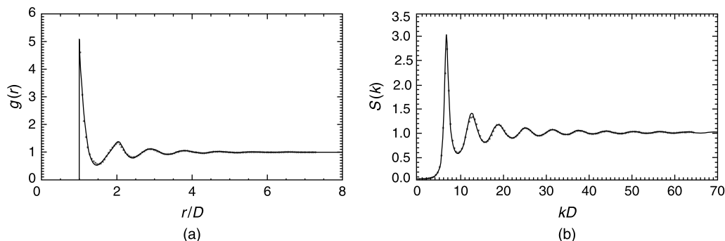
FIGURE 16.2 (a) The pair correlation function g(r) and (b) the static structure factor S(k) for a three-dimensional system of hard spheres at volume fraction \eta = 0.49 from an MC simulation of 2916 particles (M. Glaser, unpublished). This value of the volume fraction is in the liquid phase close to the solid–liquid coexistence line. The solid lines depict the pair correlation function and the static structure factor from the Percus–Yevick approximation; see Percus and Yevick (1958), Wertheim (1963), and Hansen and McDonald (1986).
