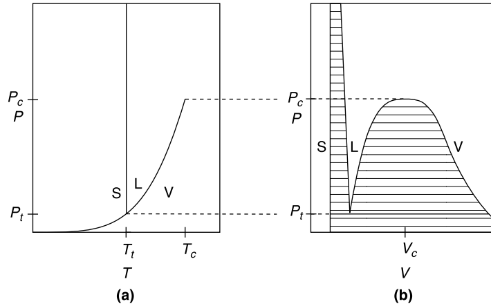
FIGURE 4.2 Sketches (not-to-scale) of the (a) P - T and (b) P - V phase diagrams for argon. This geometry is generic for a wide range of materials. The letters S, L, and V denote solid, liquid, and vapor phases.
