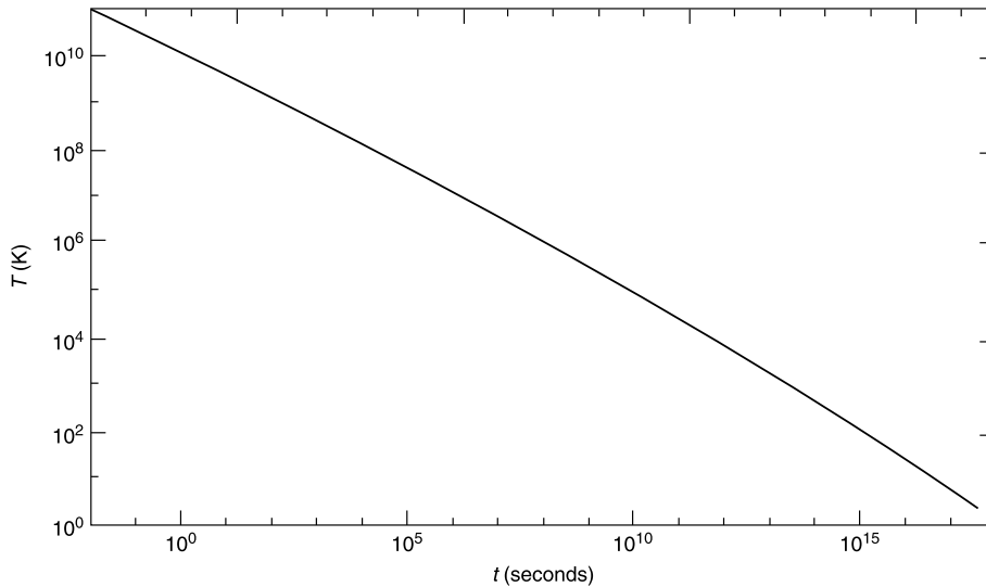
FIGURE 9.5 Sketch of the photon temperature vs. the age of the universe. At early times, radiation dominated the energy density, so T \sim t^{-1/2} . At later times ( t > 10^{13} s), nonrelativistic matter dominated the energy density, so T \sim t^{-2/3} . In the current dark energy-dominated stage, the universe is beginning to expand exponentially with time, so the photon temperature is beginning to fall exponentially.
