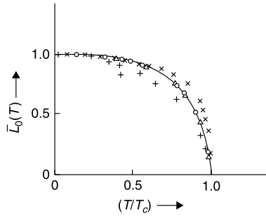
FIGURE 12.7 The spontaneous magnetization of a Weiss ferromagnet as a function of temperature. The experimental points (after Becker) are for iron ( \times ), nickel ( \circ ), cobalt ( \Delta ), and magnetite ( + ).
