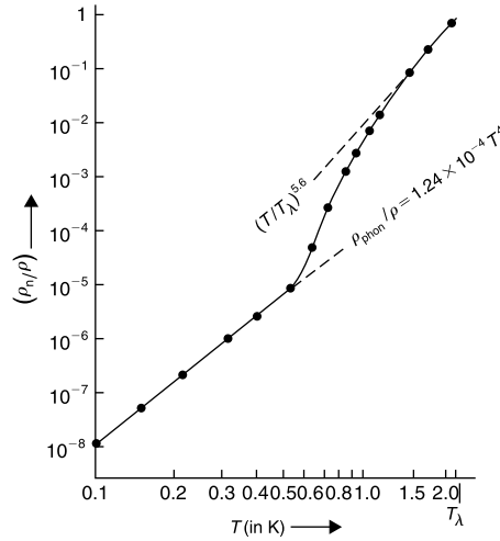
FIGURE 7.17 The normal fraction (\rho_n/\rho) , as obtained from experimental data on (i) the velocity of second sound and (ii) the entropy of liquid He II (after de Klerk et al., 1953).
