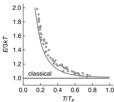
FIGURE 8.10 Experimental results for the mean energy per particle divided by the equipartition value of 3kT vs. scaled temperature ( T/T_F ) for ultracold ^{40}\text{K} atoms in a harmonic trap compared with the theoretical Fermi gas value from equations (4) and (5). This shows the development of the Fermi degeneracy of the gas at low temperatures. From Jin (2002). Figure courtesy of the IOP. Reprinted with permission; copyright © 2002 American Institute of Physics.
