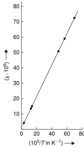
FIGURE 3.7 Plot of \chi versus 1/T for a powdered sample of copper potassium sulphate hexahydrate (after Hupse, 1942).
