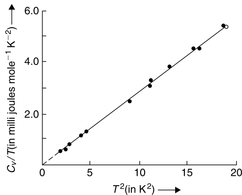
FIGURE 7.16 A plot of (C_V/T) vs. T^2 for KCl, showing the validity of the Debye T^3 -law. The experimental points are from Keesom and Pearlman (1953).
