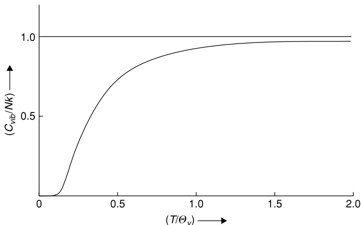
FIGURE 6.4 The vibrational specific heat of a gas of diatomic molecules. At T = \Theta_v , the specific heat is already about 93% of the equipartition value.
