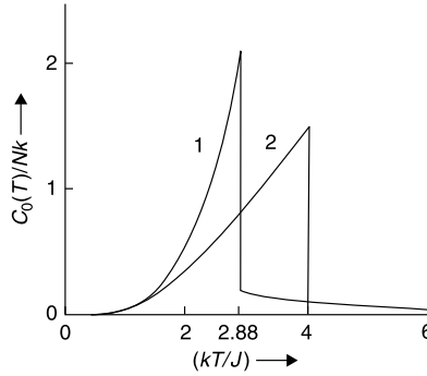
FIGURE 12.9 The field-free specific heat of an Ising lattice with coordination number 4. Curve 1 is obtained in the Bethe approximation, curve 2 in the Bragg–Williams approximation.
