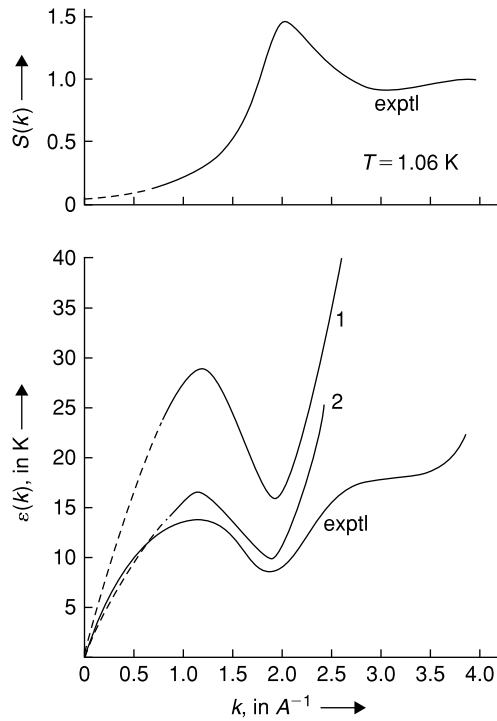
FIGURE 11.2 The energy spectrum of the elementary excitations in liquid {}^4\text{He} . The upper portion shows the structure factor of the liquid, as derived by Henshaw (1960) from experimental data on neutron diffraction. Curve 1 in the lower portion shows the energy-momentum relationship based on the Feynman formula (5), while curve 2 is based on an improved formula by Feynman and Cohen (1956). For comparison, the experimental results of Woods (1966) obtained directly from neutron scattering are also included.
