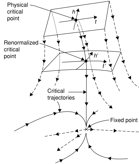
FIGURE 14.5 The parameter space of a physical system, showing critical trajectories (solid lines) flowing into the fixed point. The subspace of the relevant variables, t and h , is everywhere “orthogonal” to these trajectories (on all of which t = h = 0 ); the critical trajectories differ from one another only in respect of irrelevant variables that vanish as the fixed point is approached. The dashed lines depict that part of the flow in which the relevant variables play a decisive role.
