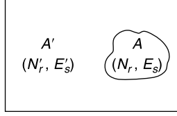
FIGURE 4.1 A statistical system immersed in a particle–energy reservoir.
