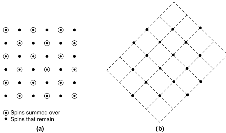
FIGURE 14.2 A scale transformation by “decimation,” with l = \sqrt{2} and d = 2 . (a) The original lattice has N (= 36) spins. (b) The transformed lattice has N' (= 18) spins. The latter is yet to be rescaled (and rotated through an angle \pi/4 ) so that it looks very much the same as the former, especially in the limit N, N' \rightarrow \infty .
