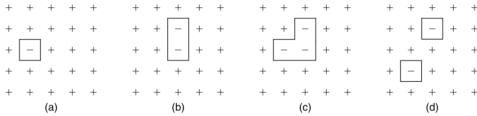
FIGURE 13.18 The lowest few excited states of the lattice. (a) The q = 2 states have a single down spin in a sea of up spins or a single up spin in a sea of down spins; these states have energy 8J above the ground state and there are g_2 = 2nm configurations. (b) The q = 3 states have a pair of down spins in a sea of up spins, or vice versa; these states have energy 12J above the ground state and g_3 = 4nm configurations. (c) and (d) The q = 4 states can have a single grouping of opposite spins or a pair of isolated flipped spins; these states have energy 16J above the ground state and the total number of configurations g_4 = (nm)^2 + 9nm .
