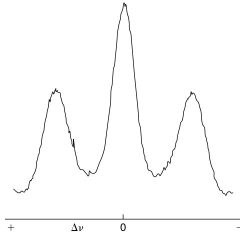
FIGURE 15.10 Dynamical structure factor for carbon tetrachloride using 632.8 nm He-Ne laser with a 90-degree scattering angle. The structure factor is symmetric since \hbar\omega \ll kT . The Landau–Placzek ratio of the integrated intensity under the Rayleigh peak to the integrated intensities under the two Brillouin peaks is related to the ratio of the constant-pressure heat capacity to the constant-volume heat capacity: I_R/(2I_B) = C_P/C_V - 1 = 0.72 \pm 0.03 (Landau and Placzek, 1934). The locations of the Brillouin peaks give the sound speed and the widths of the peaks measure the thermal diffusivity and sound attenuation coefficient of the liquid; see equation (45). From Cummins and Gammon (1966), reprinted with permission; copyright © 1966 American Institute of Physics.
