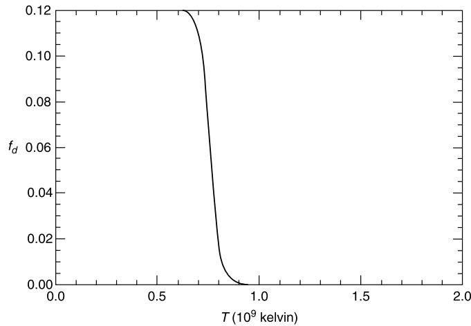
FIGURE 9.7 Plot of the equilibrium deuterium fraction f_d vs. temperature T for neutron fraction q = 0.12 and baryon-to-photon ratio \eta = 6 \times 10^{-10} . As T falls below about 6 \times 10^8 K the neutrons are nearly all bound into deuterons. Further two-body reactions convert most of the deuterium into heavier nuclei, primarily {}^4\text{He} .
