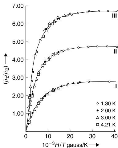
FIGURE 3.9 Plots of \bar{\mu}_z/\mu_B as a function of H/T . The solid curves represent the theoretical results, while the points mark the experimental findings of Henry (1952). Curve I is for potassium chromium alum ( J = \frac{3}{2}, g = 2 ), curve II for iron ammonia alum ( J = \frac{5}{2}, g = 2 ), and curve III for gadolinium sulphate octahydrate ( J = \frac{7}{2}, g = 2 ).
