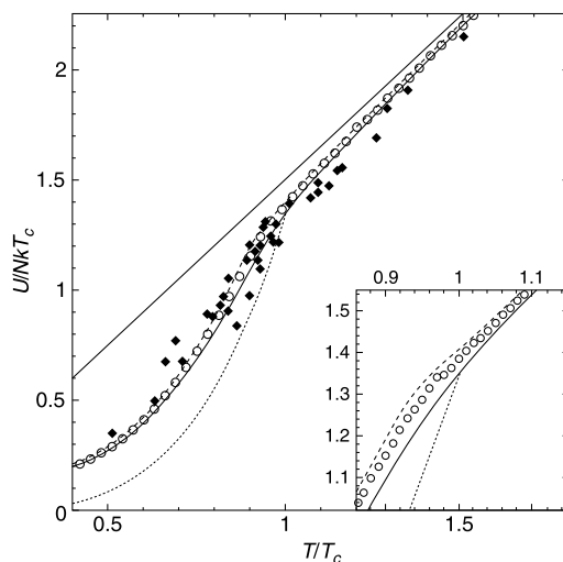
FIGURE 7.12 Comparison of the experimental measurements of Ensher et al. (1996) (diamonds) with the non-interacting internal energy result – see equation (19) and Figure 7.10(b) – (dotted curve), the zero-order solution including interactions (full curve), first-order perturbative treatment (dashed curve), and numerical solution (circles). The straight line is the classical Maxwell–Boltzmann result. The inset is an enlargement of the region around the critical temperature. The break in slope is an indication of the discontinuity in the thermodynamic limit specific heat shown in Figure 7.11. From Minguzzi et al. (1997). Reprinted with permission; copyright © 1997 American Institute of Physics.
