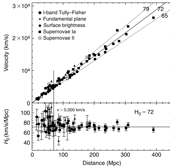
FIGURE 9.1 Hubble diagram of the spectral redshift velocity of relatively nearby galaxies vs. their distance using several astronomical standard candles. The velocity is in km/s and the distance is measured in megaparsecs, where 1 \text{ Mpc} = 3.26 \times 10^6 \text{ light years} . The best fit to the data gives a value of the Hubble parameter as H_0 = 72 \pm 8 \text{ km s}^{-1} \text{ Mpc}^{-1} . The Hubble parameter has been recently updated by Riess et al. (2009) to give H_0 = 74.2 \pm 3.6 \text{ km s}^{-1} \text{ Mpc}^{-1} . The figure is from Freedman et al. (2001) and is reproduced by permission of the AAS.
