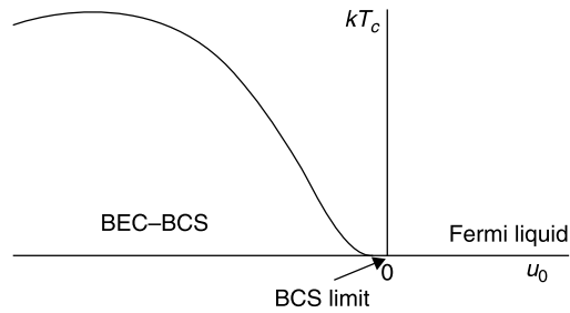
FIGURE 11.7 Sketch of the Bose–Einstein condensation–Bardeen–Cooper–Schrieffer (BEC–BCS) phase diagram on the BCS side of the Feshbach resonance for ultracold fermions in an atomic trap. The scattering length a and coupling u_0 = 4\pi\hbar^2 a/m can be tuned from positive values to negative with the help of a magnetic field. Positive (repulsive) couplings result in a Fermi liquid. Negative (attractive) couplings result in BCS condensation at low temperatures. The nature of the condensed phase varies smoothly from BCS behavior for small negative coupling to Bose–Einstein behavior for large negative coupling. The phase transition temperature has a maximum at intermediate coupling.
