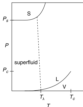
FIGURE 4.3 Sketch of the P - T phase diagram for helium-4. The letters S, L, and V denote solid, liquid, and vapor phases. The critical point is T_c = 5.19 K and P_c = 227 kPa = 2.24 atm. The solid-liquid coexistence curve starts at P_s = 2.5 MPa = 25 atm at T = 0 K and does not intersect the liquid-vapor coexistence curve. The \lambda -line is the continuous phase transition between the normal liquid and the superfluid phase. The superfluid phase transition temperature at the liquid-vapor coexistence line is T_\lambda = 2.18 K.
