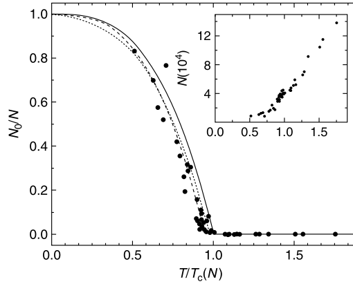
FIGURE 7.7 Experimental measurement of the Bose-condensed fraction vs. temperature, as compared with equation (8). The scaled temperature on the horizontal axis is the temperature divided by the N -dependent critical temperature given in equation (6). The inset shows the total number of atoms in the trap after the evaporative cooling. From Ensher et al. (1996). Reprinted with permission; copyright © 1996 American Physical Society.
