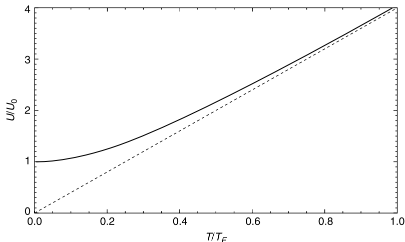
FIGURE 8.9 Scaled internal energy ( U/U_0 ) vs. scaled temperature ( T/T_F ) for an ideal Fermi gas in a harmonic trap from equations (4) and (5). The dotted line is the corresponding classical result U(T) = 3NkT .
