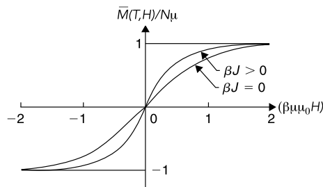
FIGURE 13.4 The degree of magnetization of an Ising chain as a function of the parameter (\beta\mu\mu_0 H) .
