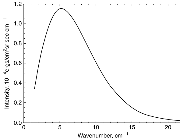
FIGURE 9.2 Cosmic microwave background spectrum from COBE fit numerically to the Planck distribution with an average temperature T = 2.725 \pm 0.002 \text{ K} ; see equations (7.3.8) and (7.3.9) and Figure 7.13. The error bars at the 43 equally spaced frequencies from the Far Infrared Absolute Spectrophotometer (FIRAS) data are too small to be seen on this scale. Figure courtesy of NASA.
