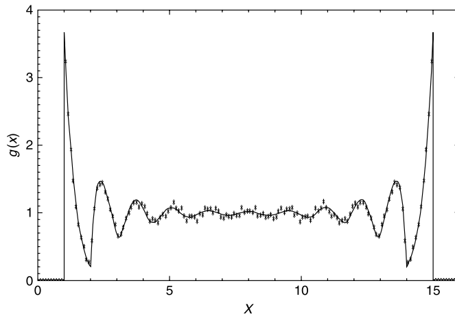
FIGURE 13.1 The pair correlation function for a system of 12 hard disks on a ring with scaled number density nD = 0.75 . The solid line represents the exact solution from equations (6) and (7), as compared with a Monte Carlo simulation.
