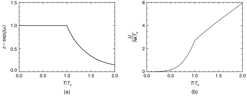
FIGURE 7.10 (a) Fugacity and (b) scaled internal energy vs. scaled temperature ( T/T_c ) for a Bose–Einstein condensate in a harmonic trap.
