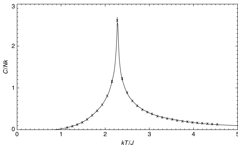
FIGURE 16.1 MC specific heat ( \times 's) of the two-dimensional Ising model on a 128 \times 128 lattice, as compared with the exact solution (solid line) from Section 13.4.A; see Kaufman (1949), Ferdinand and Fisher (1969) and Beale (1996). The MC error bars are smaller than the symbols used, except near the bulk critical temperature T_c(\infty) . Each data point represents an average using 10^5 MC sweeps, except at the bulk critical point, where 10^6 MC sweeps were used to mitigate critical slowing down.
