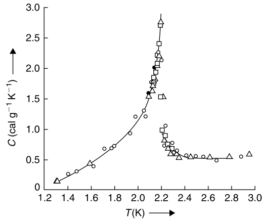
FIGURE 7.5 The specific heat of liquid {}^4\text{He} under its own vapor pressure (after Keesom and coworkers).
