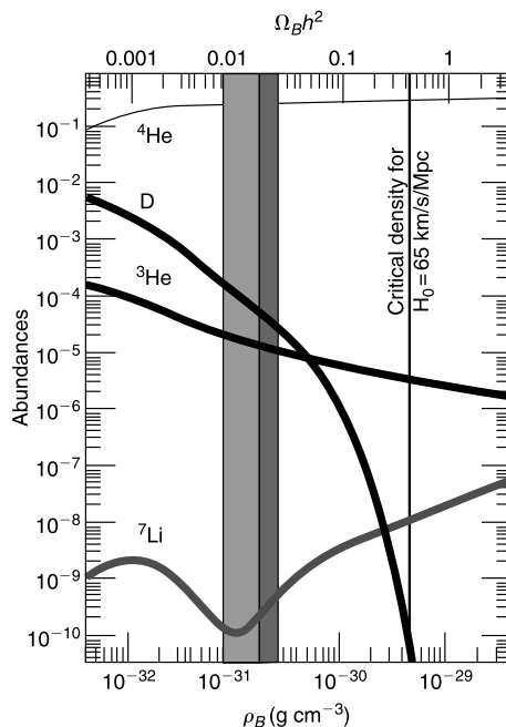
FIGURE 9.4 Calculated primordial abundances of light elements ( {}^4\text{He} , \text{D} \equiv {}^2\text{H} , {}^3\text{He} , and {}^7\text{Li} ) as functions of the baryon-to-photon ratio. The baryon-to-photon ratio is given by \eta = 2.7 \times 10^{-8} \Omega_B h^2 , where h is the Hubble parameter in units of 100 \text{ (km/s)/Mpc} and \Omega_B = 0.046 is the current baryonic fraction of the mass-energy density of the universe; see Copi et al. (1997), Schramm and Turner (1998), and Steigman (2006). The experimentally allowed range is in the gray vertical bands. From Schramm and Turner (1998). Reprinted with permission; copyright © 1998 American Physical Society.
