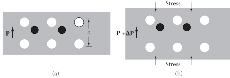
Figure 23 (a) Unstressed ferroelectric crystal and (b) stressed ferroelectric crystal. The stress changes the polarization by \Delta\mathbf{P} , the induced piezoelectric polarization.
