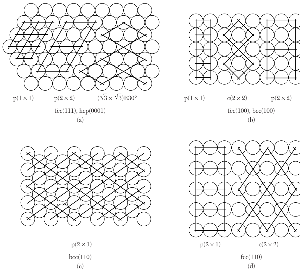
Figure 2 Surface nets of adsorbed atoms. The circles represent atoms in the top layer of the substrate. In (a) the designation \text{fcc}(111) means the (111) face of an fcc structure. This face determines a reference net. The lines represent ordered overlayers, with adatoms at the intersections of two lines. The intersection points represent diperiodic nets (lattices in two dimensions). The designation p(1 \times 1) in (a) is a primitive mesh unit for which the basis is identical with the basis of the reference net. In (b) the c(2 \times 2) mesh unit is a centered mesh with basis vectors twice as long as those of the reference net. Atomic adsorption on metals takes place most often into those surface sites (hollow sites) that maximize the number of nearest-neighbor atoms on the substrate. (After Van Hove.)
