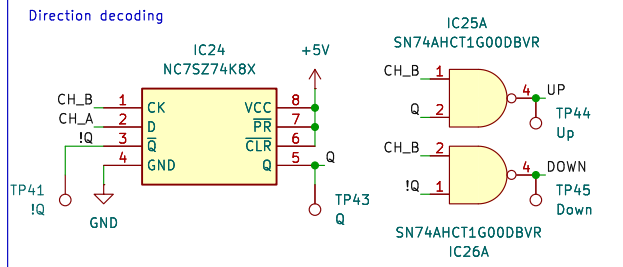
Direction decoding
