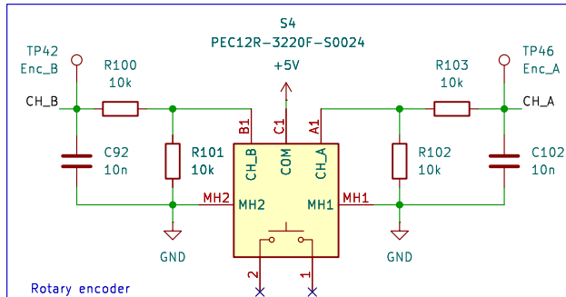
Direction decoding
