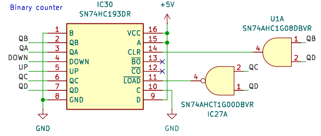
Binary counter
