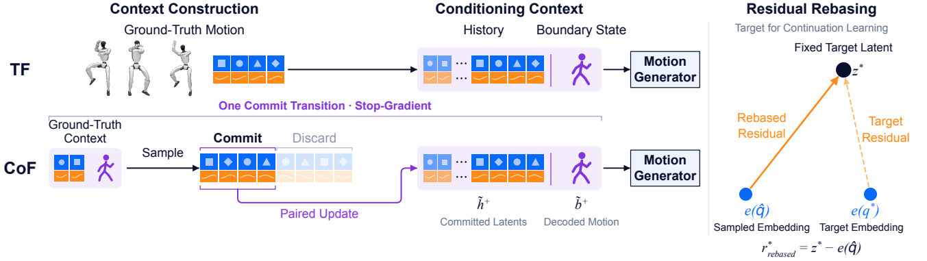
Fig. 3. Constructing continuation contexts with Commit Forcing. TF uses ground-truth history and boundary state. CoF constructs one commit transition under stop-gradient: committed latents update history, and decoded motion determines the paired boundary state for continuation learning. Residual rebasing keeps z^* fixed and forms r_{rebased}^* = z^* - e(\hat{q}) without re-encoding ground-truth motion at the generated boundary. G1 poses, tile counts, and geometry are schematic.
