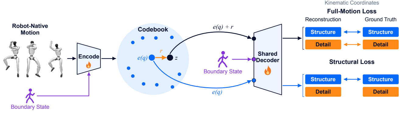
Fig. 2. Learning complementary structure and detail. Core paired reconstruction objectives. The encoder maps robot-native motion and its boundary state to a latent composed of codebook embedding e(q) and continuous residual r . The shared decoder is evaluated twice with the same boundary state, using e(q) + r and e(q) . Both paths reconstruct complete motion. Blue and orange bands denote structural and complementary kinematic coordinates, including velocities; comparison links indicate which subsets enter each loss. Full-motion supervision constrains both subsets, whereas structural supervision constrains only blue. G1 poses, codebook geometry, and band widths are schematic; flames mark learned modules.
