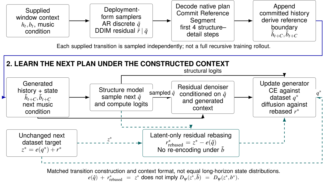
Fig. 6. Commit Forcing transition construction and supervision. A sampled, jointly committed structure–detail segment supplies the next history and reference boundary. The next dataset latent remains fixed; residual rebasing expresses it relative to the sampled next structure. This preserves the latent target, while the changed boundary can change its decoded motion. The two stages are constructed independently for each supplied training example.
