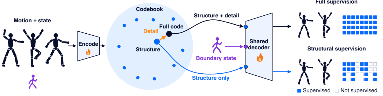
Fig. 2. Learning complementary structure and detail. The codebook anchor and continuous offset form the full code. Both paths share one state-conditioned decoder and produce complete motions. Filled cells select coordinates for supervision in four blocks: native motion, native velocity, Cartesian position, and Cartesian velocity. Counts are schematic; flames mark learned modules.
