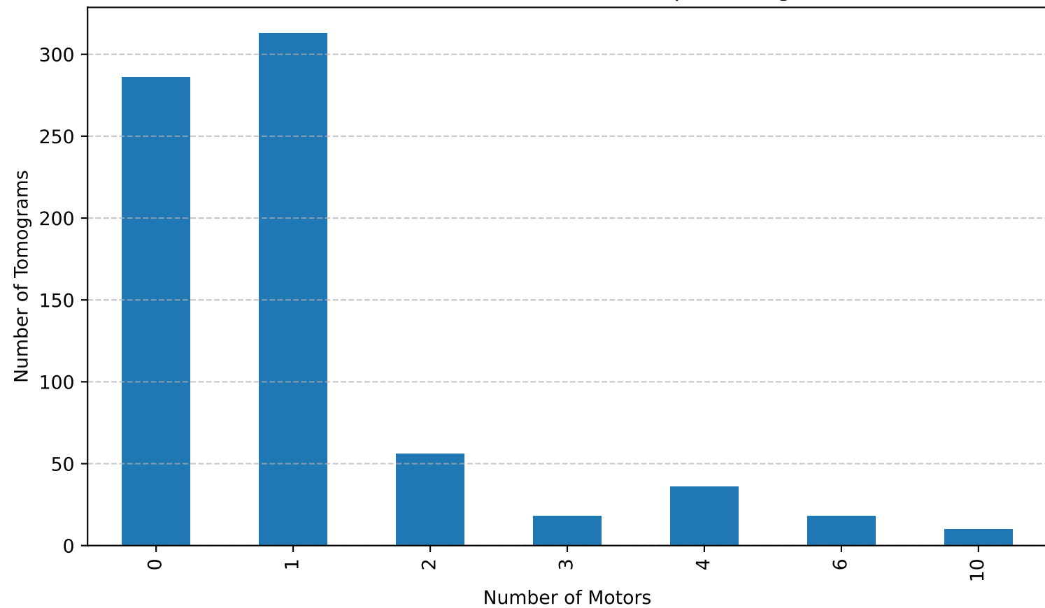
Distribution of Number of Motors per Tomogram
