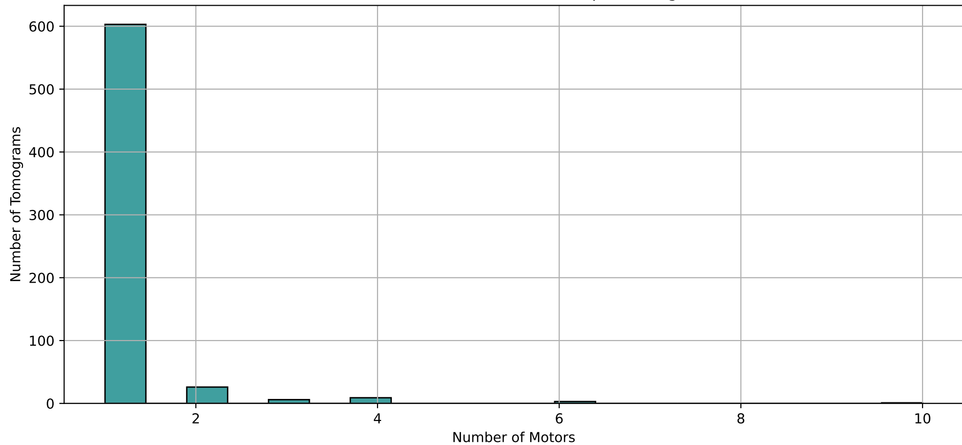
Distribution of Number of Motors per Tomogram
