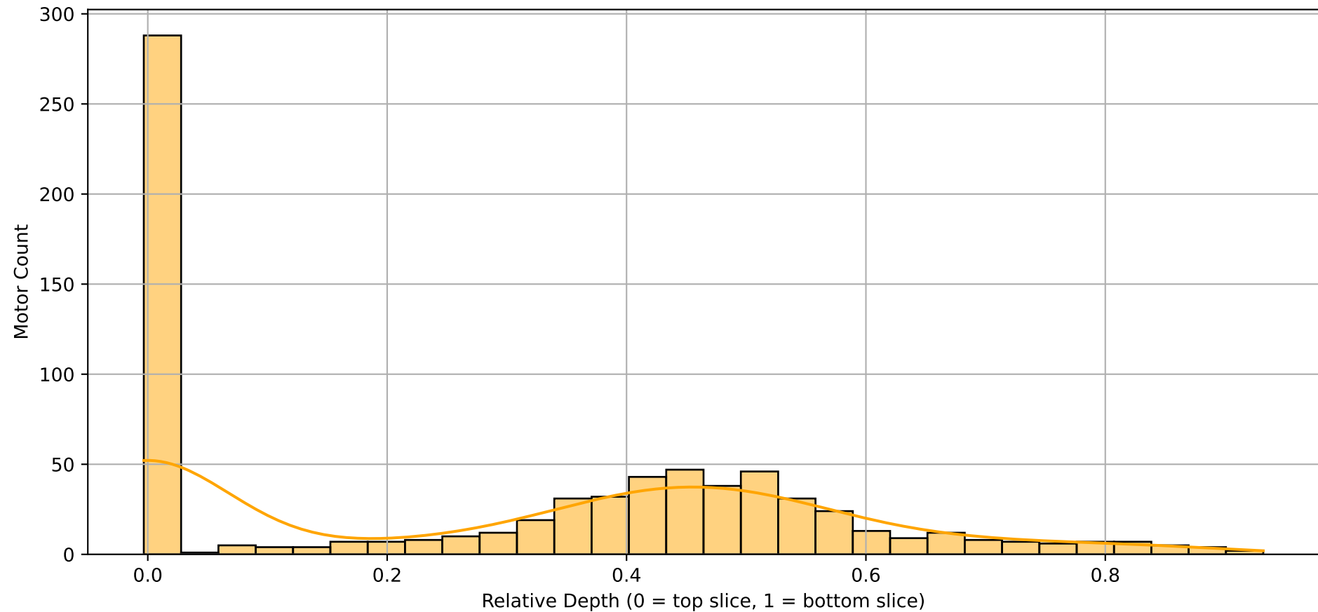
Normalized Z-Coordinate of Motors
