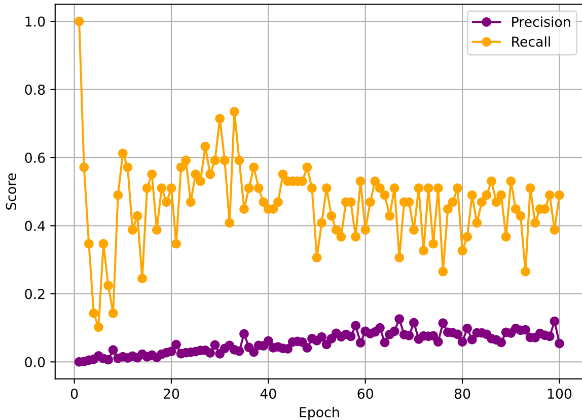
sigma12 - Precision vs Recall over Epochs
