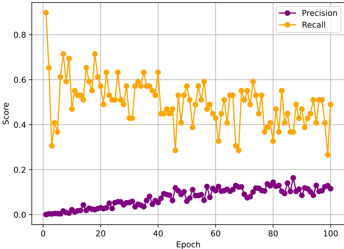
sigma16 - Precision vs Recall over Epochs
