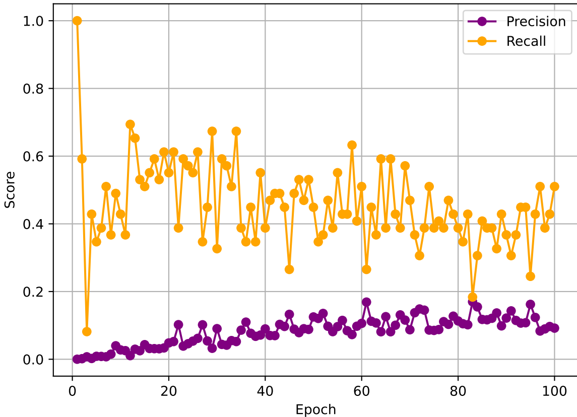
sigma8 - Precision vs Recall over Epochs
