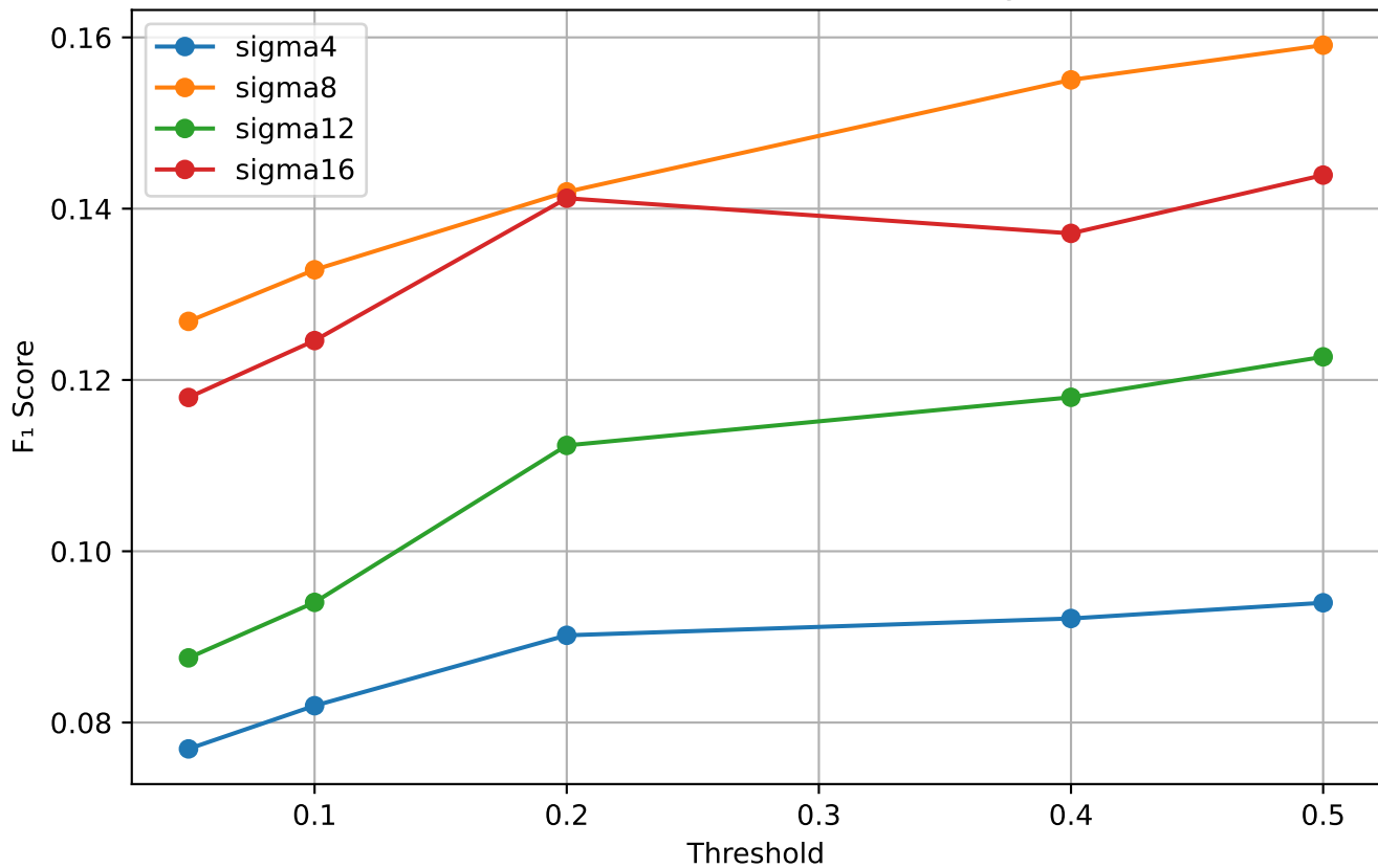
Overall F 1 across thresholds and sigmas
