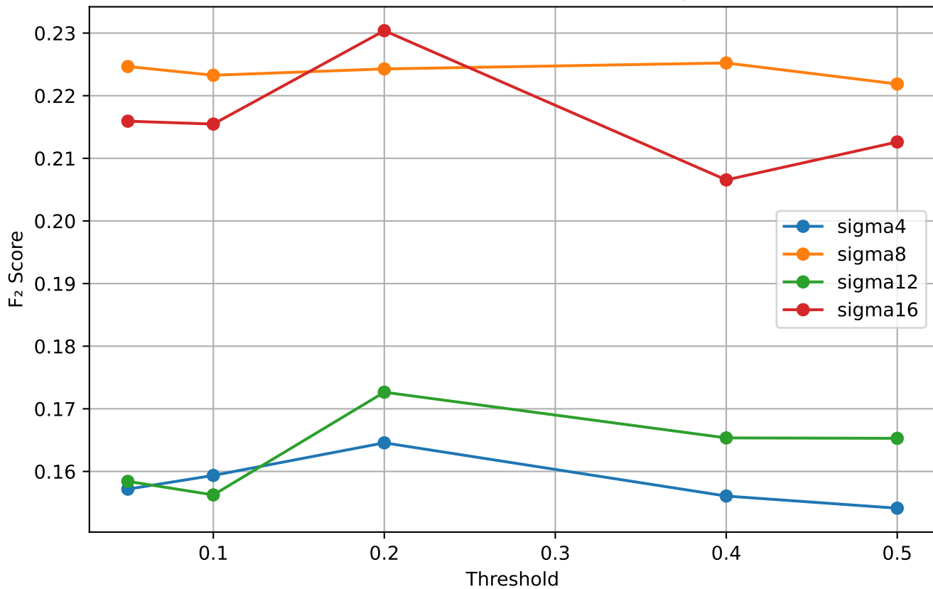
Overall F 2 across thresholds and sigmas
