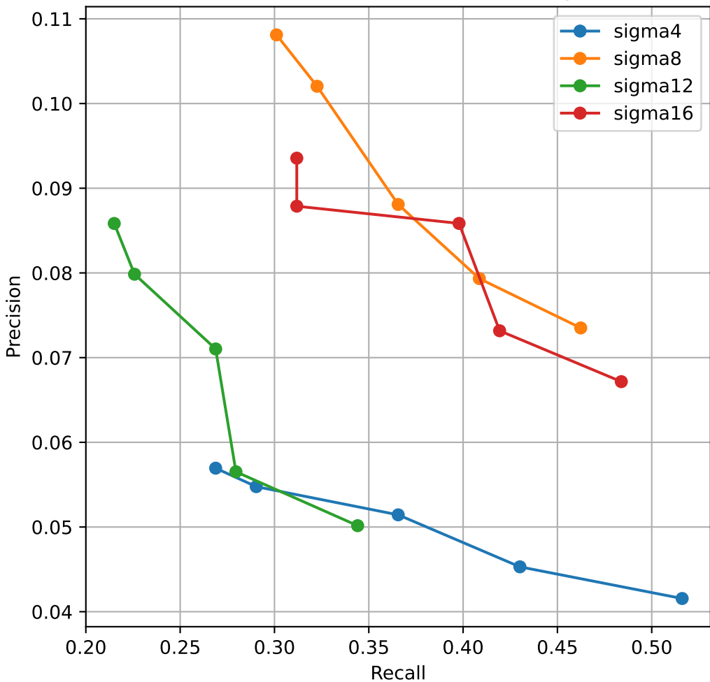
Precision-Recall trade-off across sigmas
