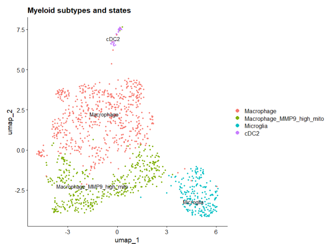
Figure 17. Myeloid subtype characterization and M1/M2 polarization states. UMAP embedding of high-resolution sub-clustered myeloid populations identifying Macrophages, Macrophage_MMP9_high_mito, Microglia, and cDC2s.
