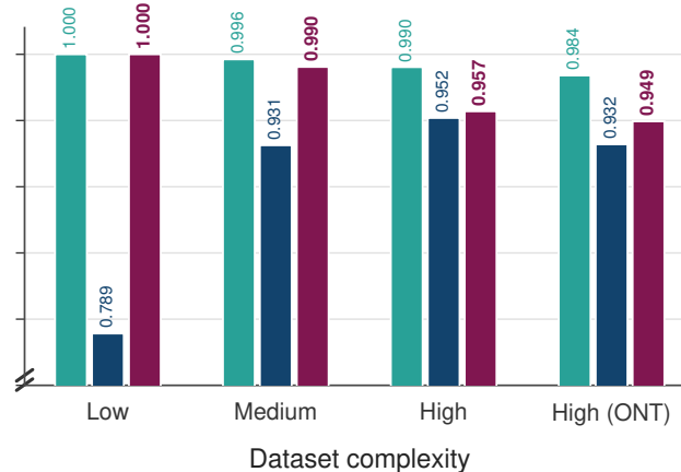
(b) Recall
