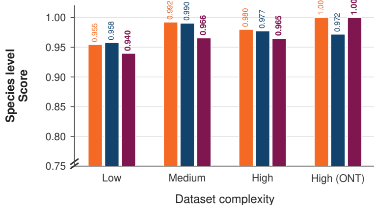
(a) Precision
