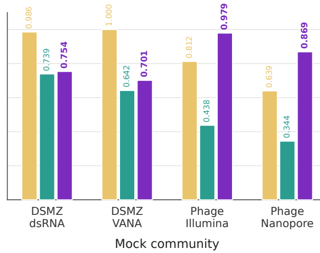
(b) Recall
