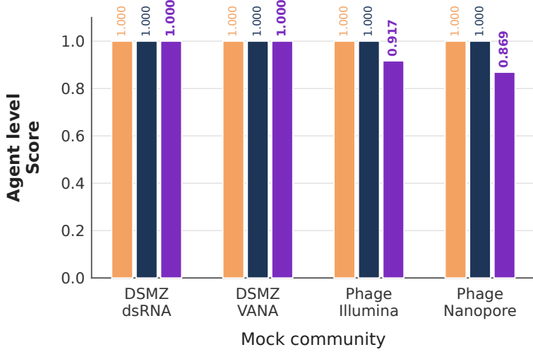
(a) Precision
