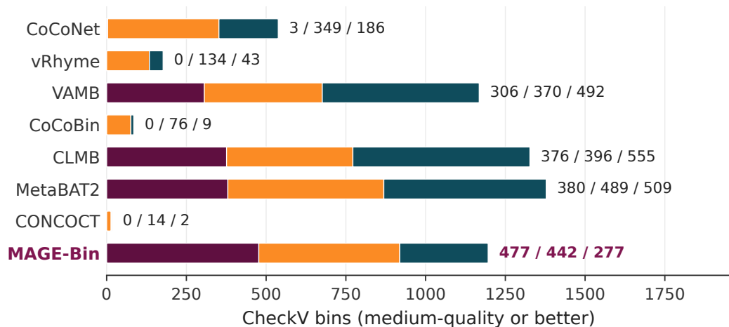
(c) Wastewater (metaFlye)
