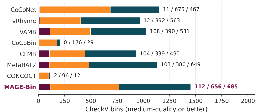
(b) Lake water (MEGAHIT)
