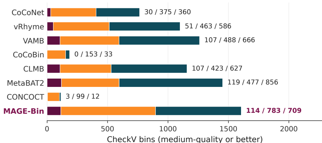
(a) Lake water (metaSPAdes)
