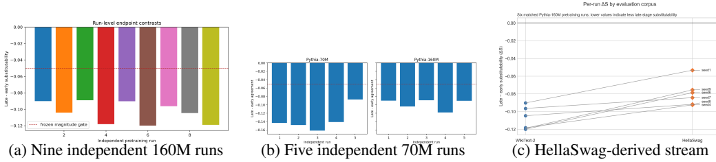
Figure 1: Empirical base. The endpoint direction repeats across independent runs, two small scales, and two evaluation streams. Panels reuse sealed ARC figures without recomputing outcomes. Differences in magnitude are not interpreted as invariance or a scaling law.
