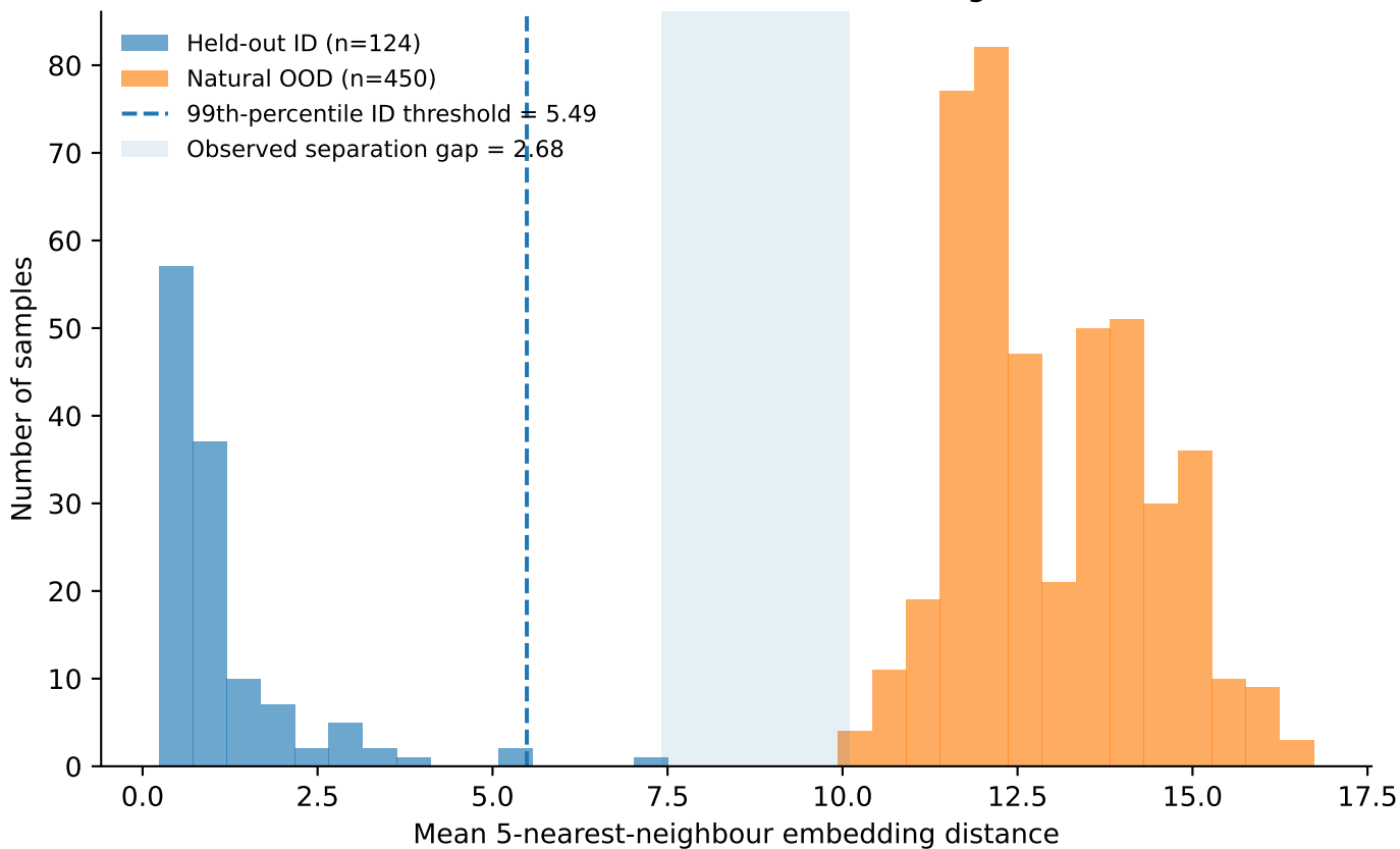
Held-out ID and Natural-OOD Embedding Distances
