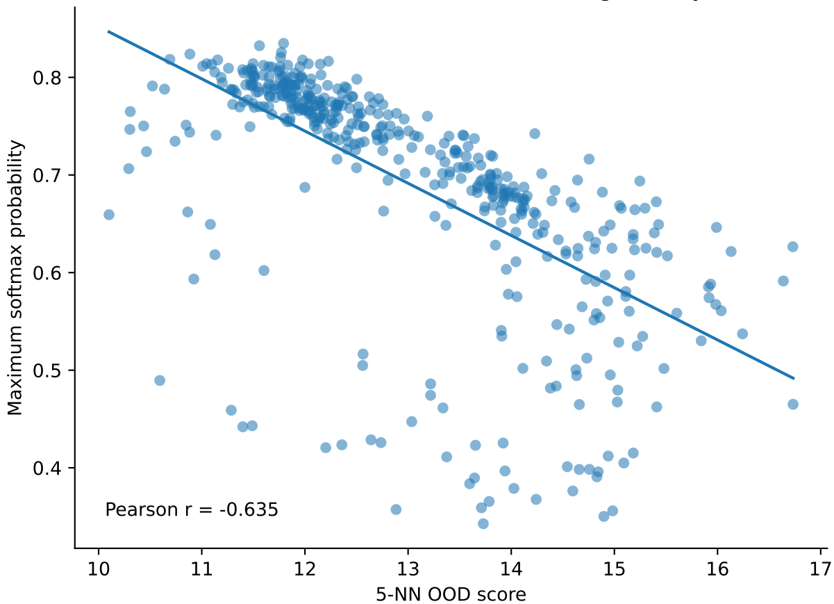
Closed-Set Confidence vs Embedding Novelty
