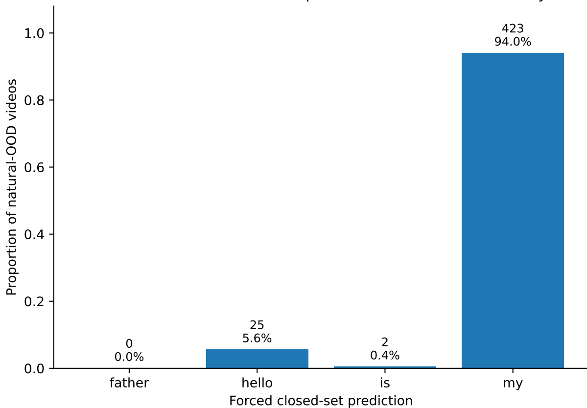
Closed-Set Prediction Collapse on Unseen KSL Vocabulary
