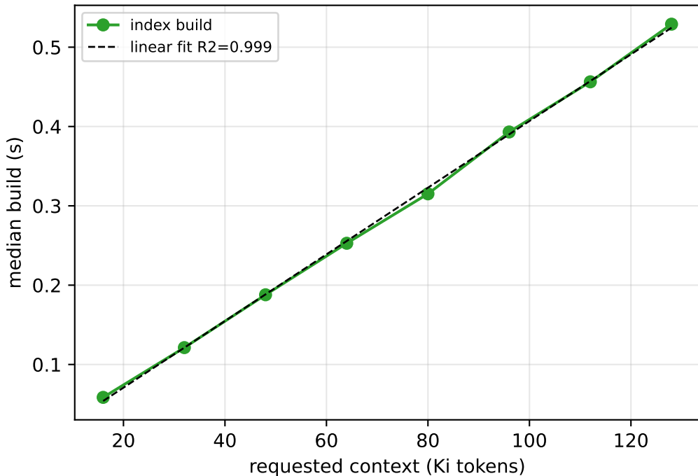
One-time index build is linear in n
