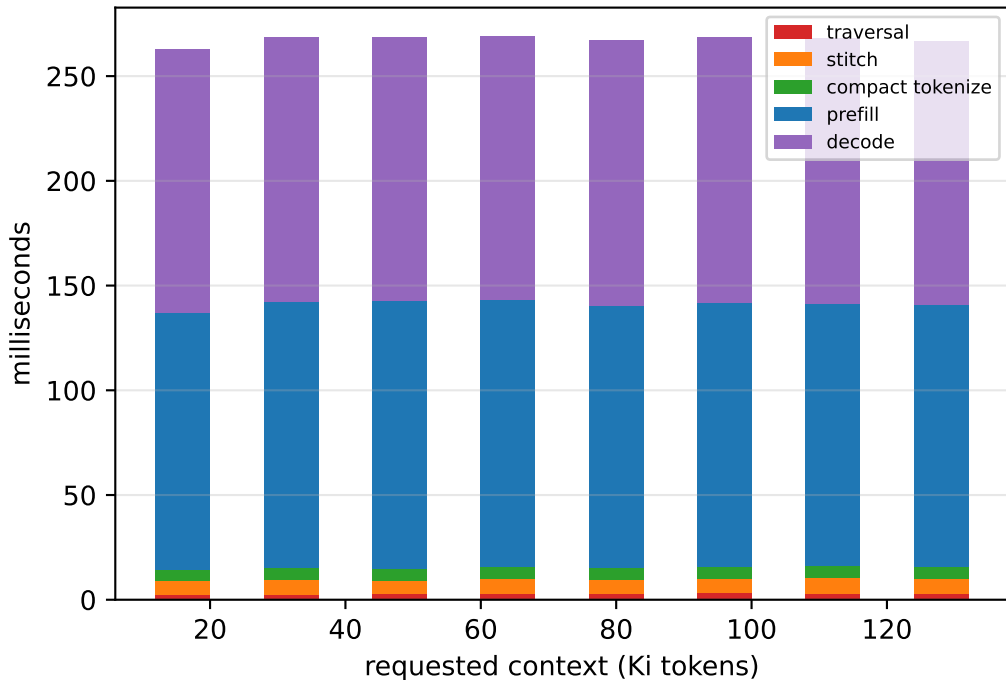
Cached query composition
