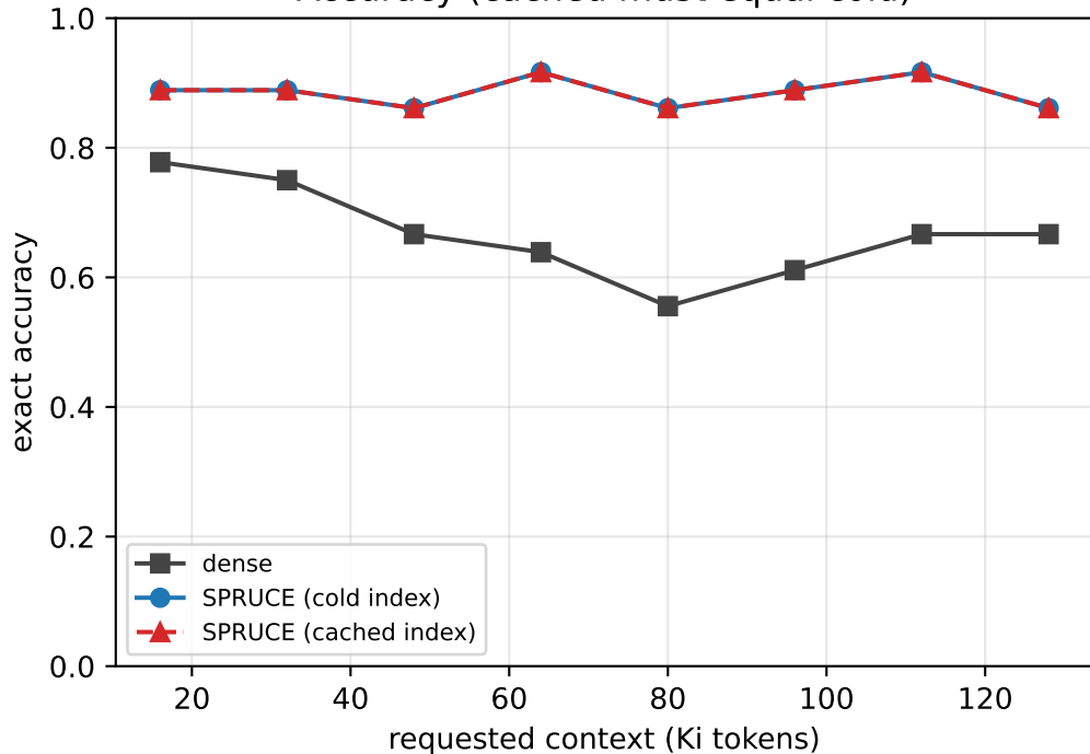
Accuracy (cached must equal cold)
