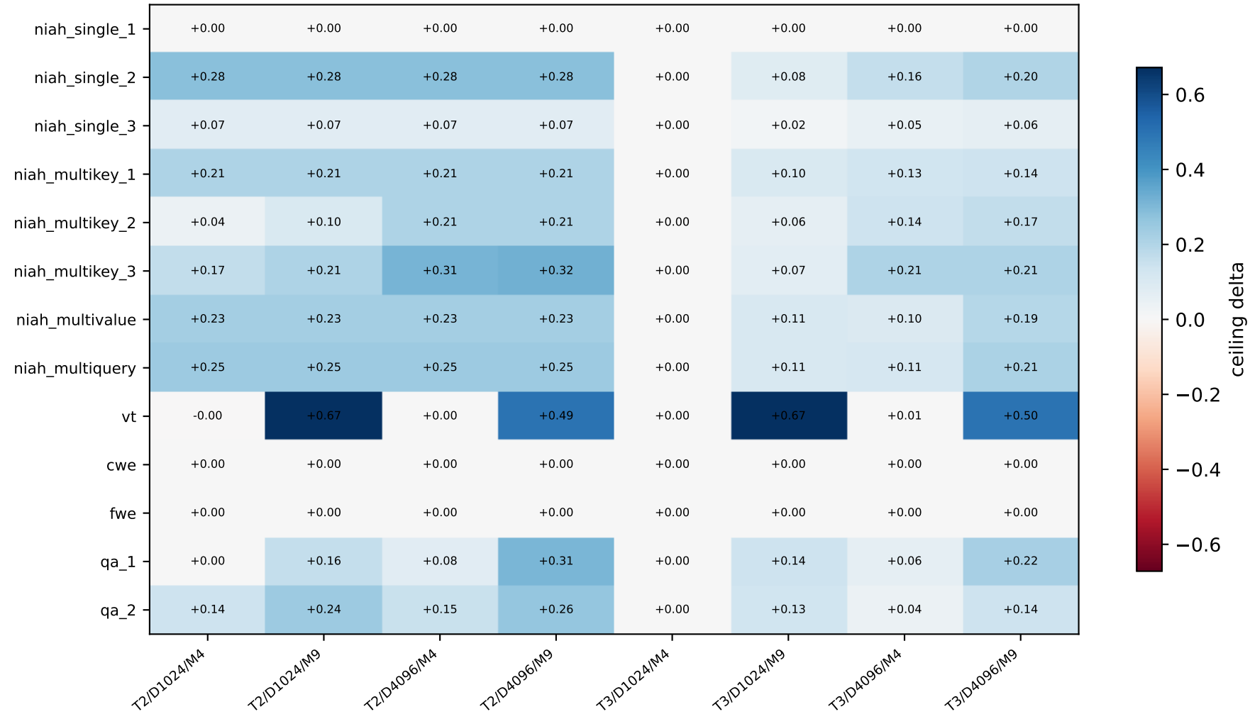
Ceiling delta by task versus T3_D1024_M4
