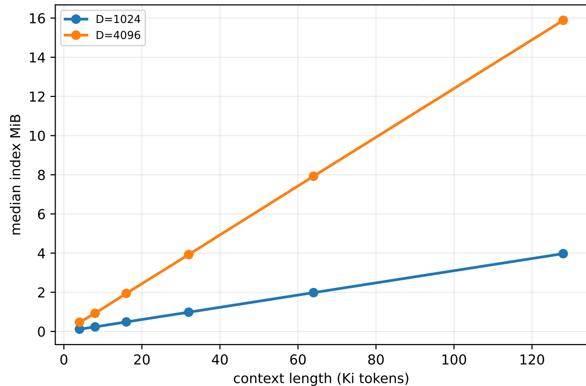
Cached lexical-index storage
