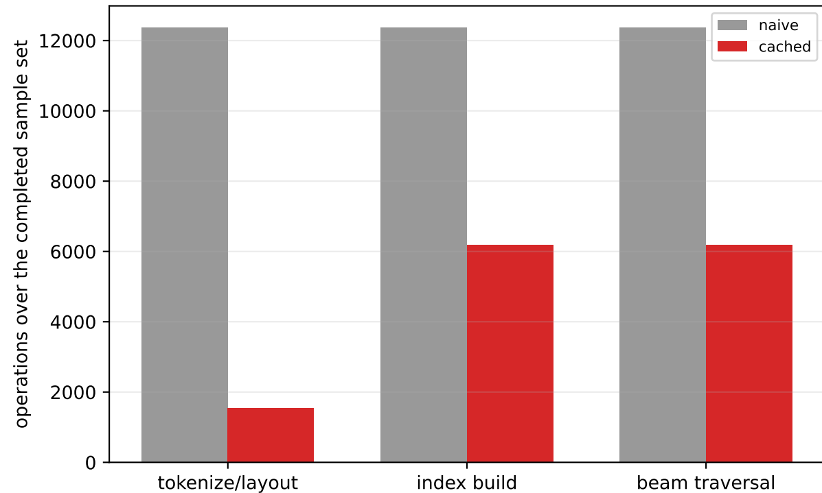
Work eliminated by exact query-independent caching
