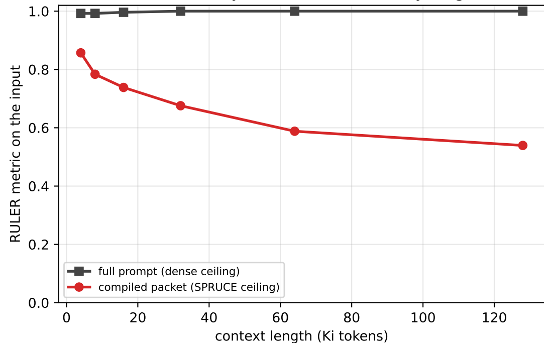
Best score any model could reach, by length
