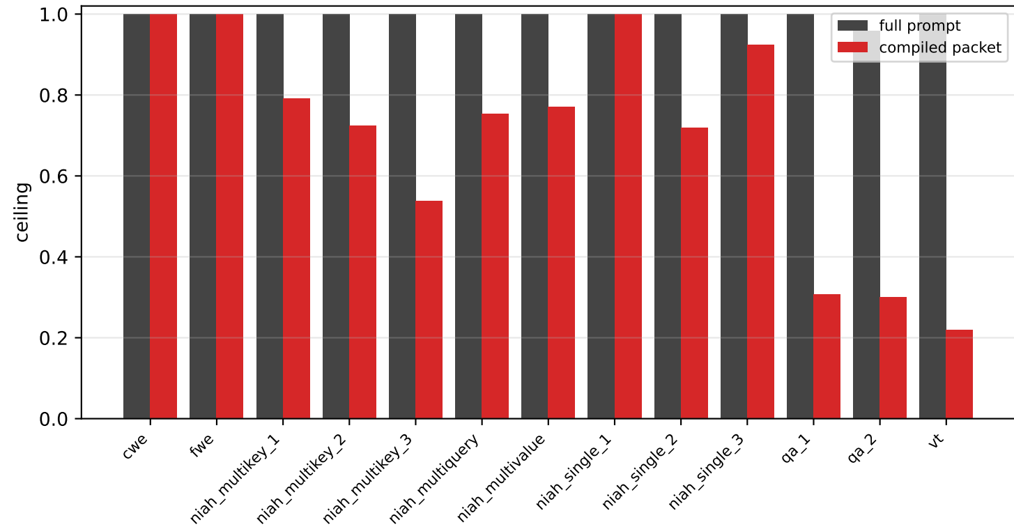
Compiler ceiling by task
