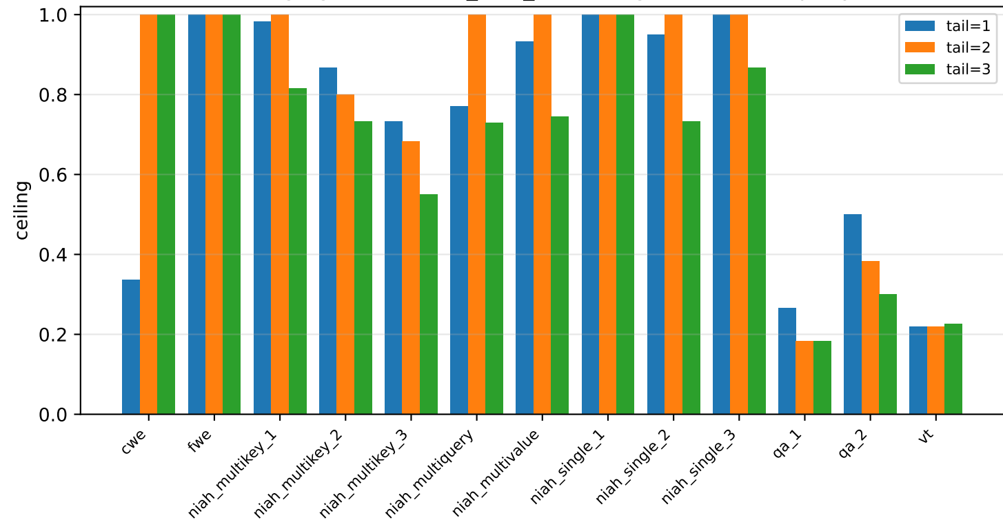
Ceiling against QUERY_TAIL_LINES (higher = better query)
