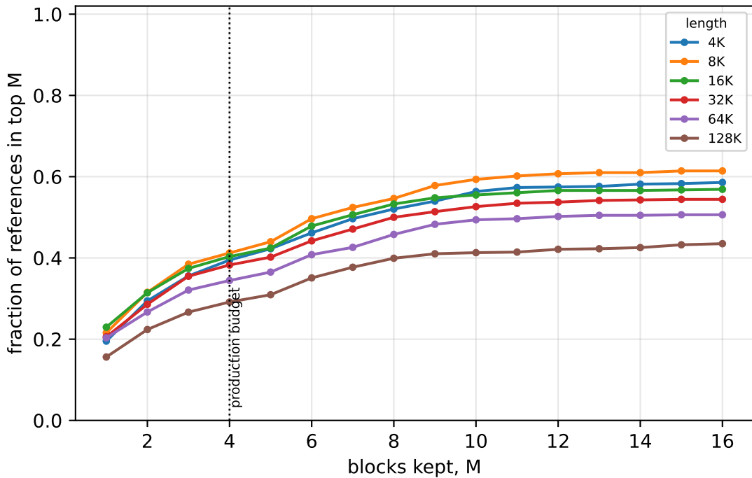
Selector recall@M (no block radius, ranked leaves only)
